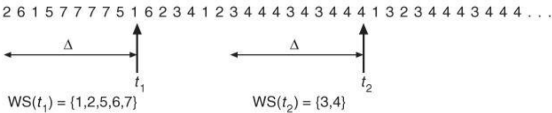
Figure 4.41 - Working-set model.
